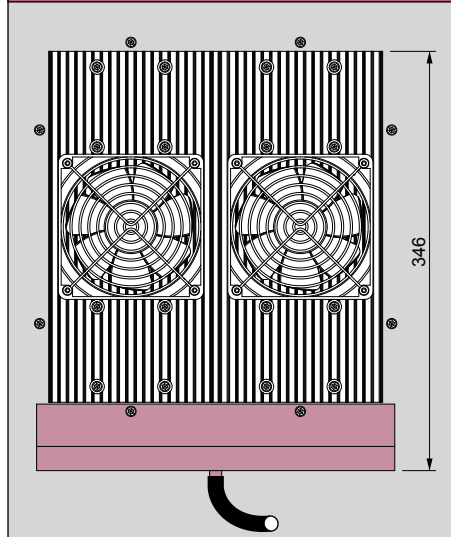
TCU200 / TCU200AC max. height with drip tray
