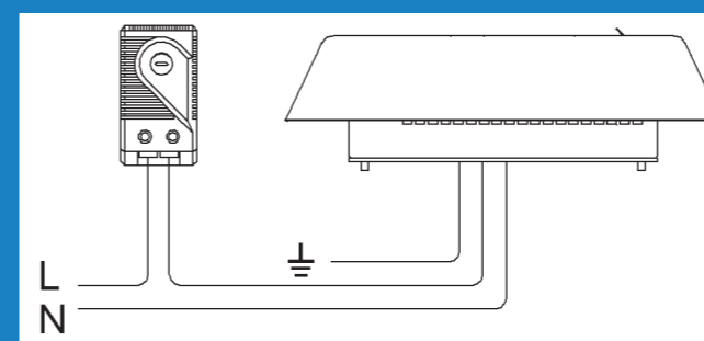
Control scheme for a roof-mount fan using AAFTO12 thermostat
