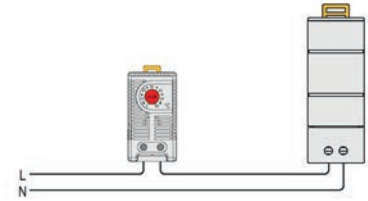
CONNECTION EXAMPLES
